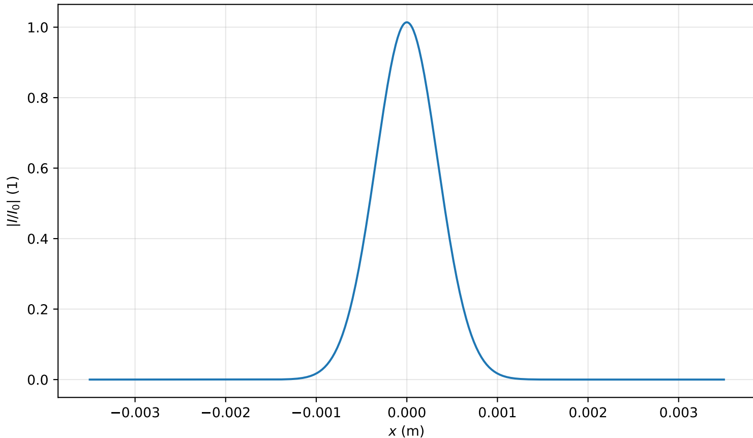
Intensity profile I(x, y = 0, z = 0.159m)/I_0 , P_{in}=0.8P_{cr} , artificial time
